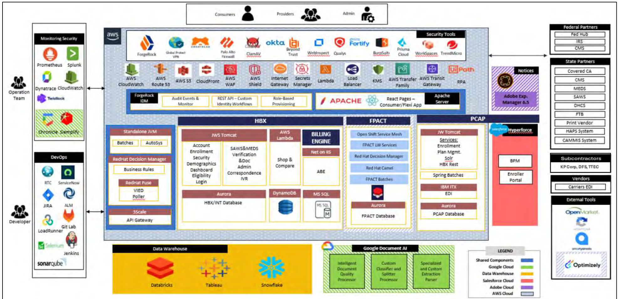
Figure 3-3: CalHEERS Architecture
