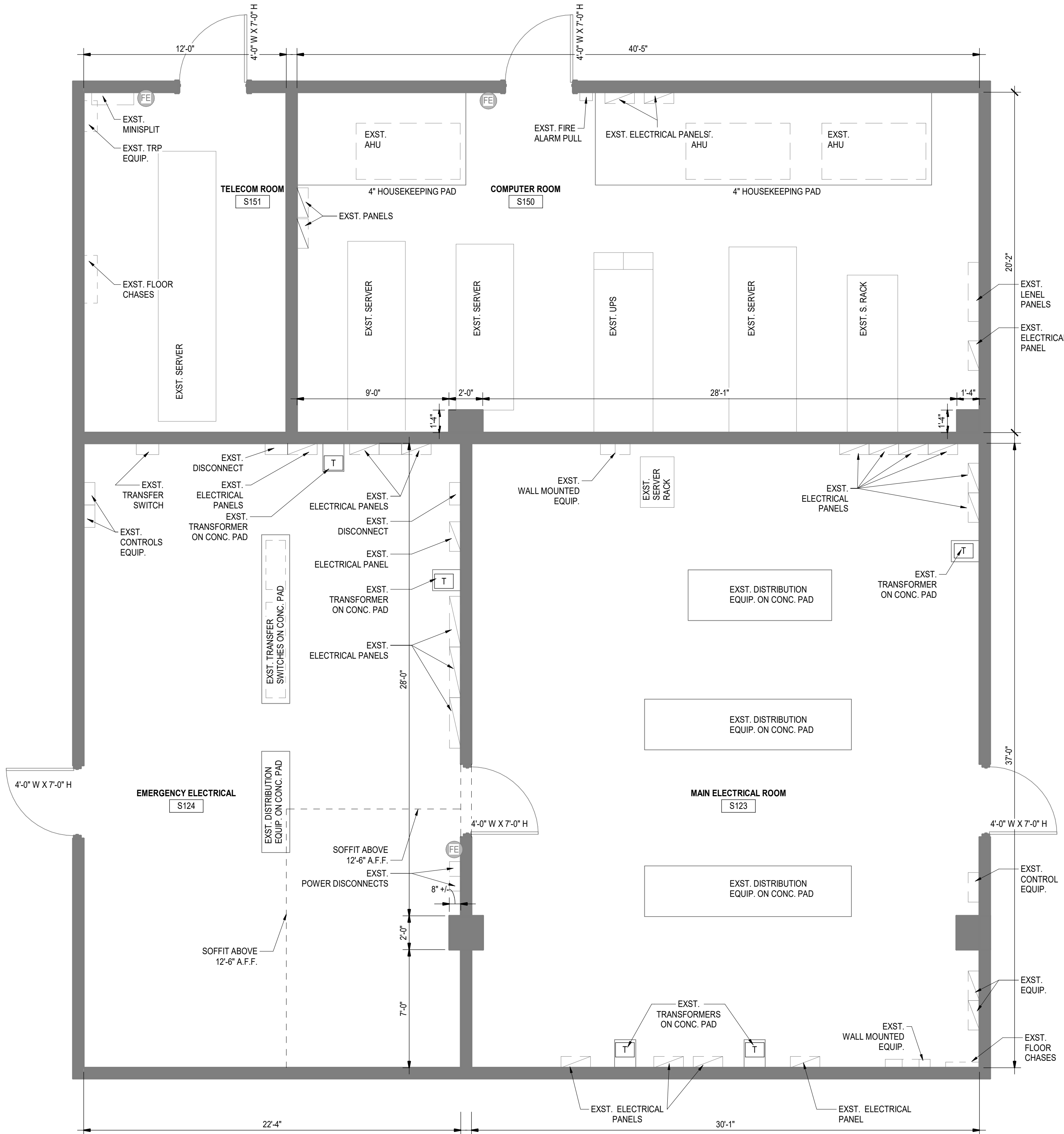
1 EXISTING FLOOR PLAN A-100 | 1/4" = 1'-0"
