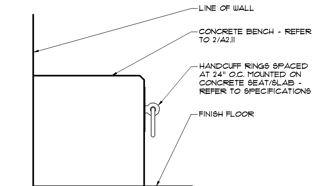
2 A102 Handcuff Ring Detail SCALE | 1/2" = 1'-0"
