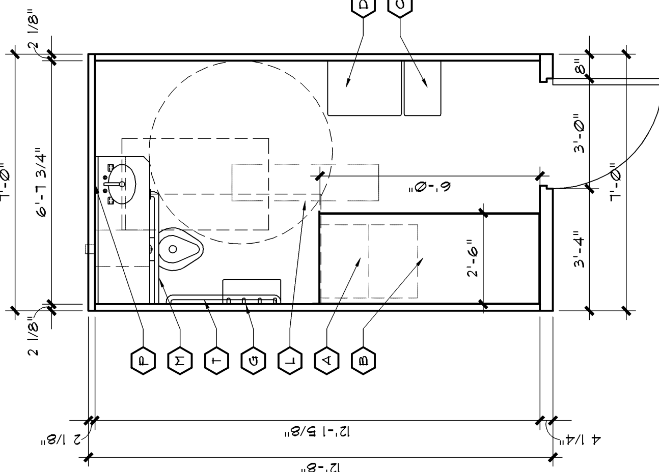
Direct Supervision ADA Accessible Cell
