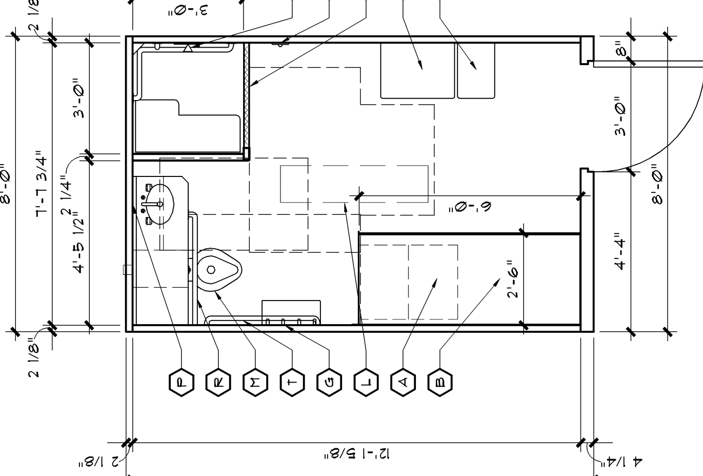
Indirect Supervision ADA Accessible Cell
