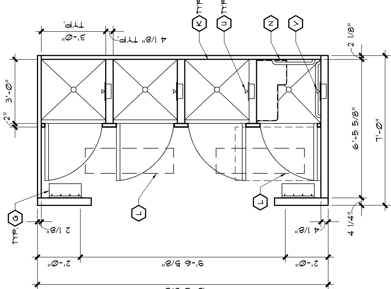
Direct Supervision ADA Accessible Shower Cell
