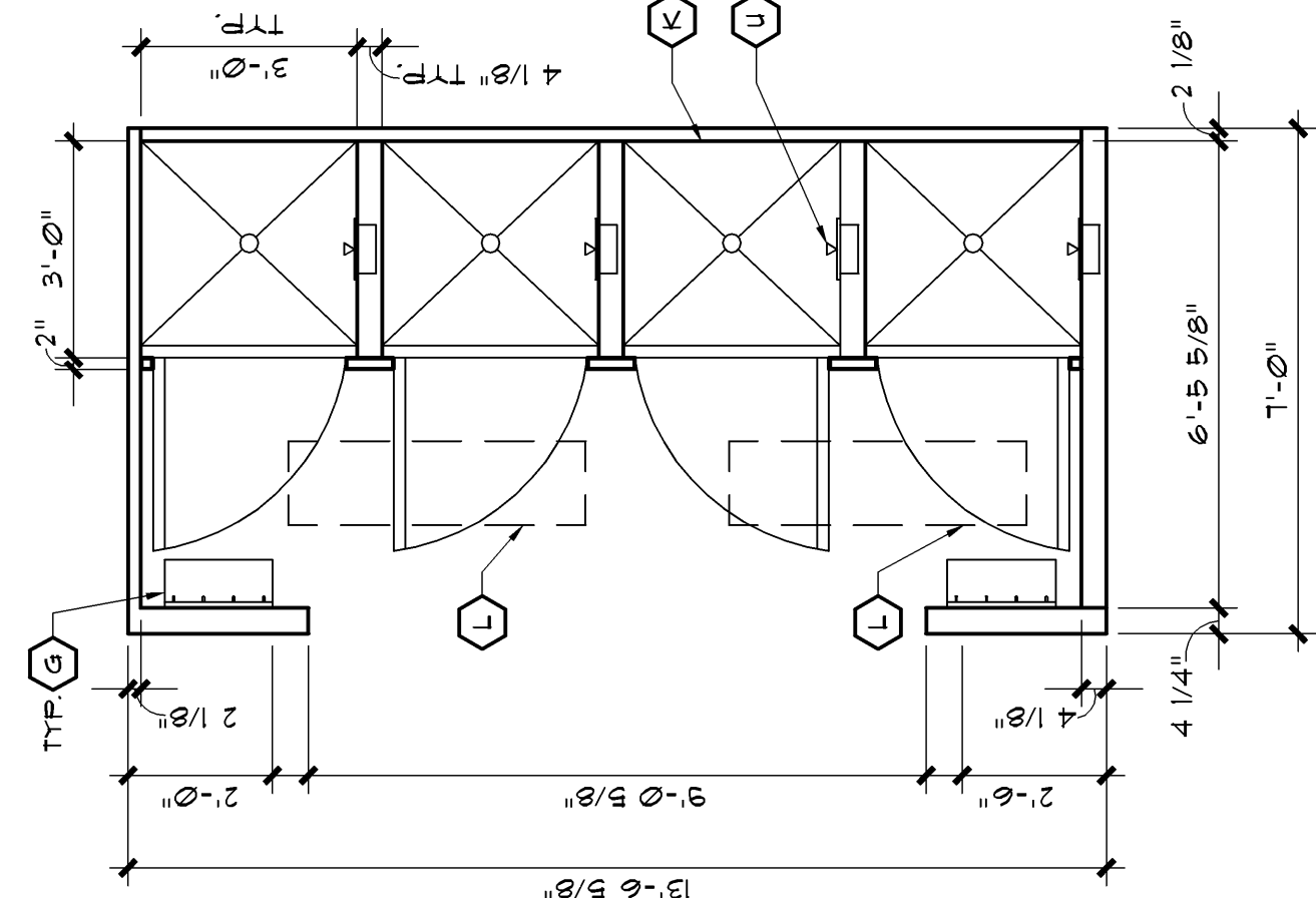
Direct Supervision Standard Shower Cell
