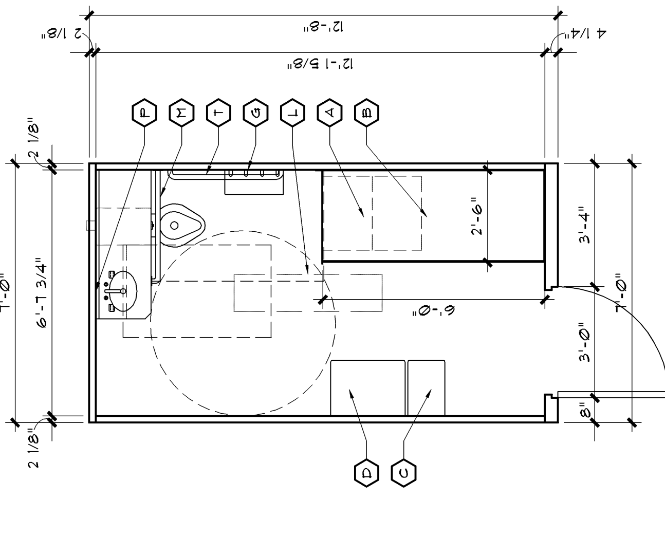
Direct Supervision ADA Accessible Cell
