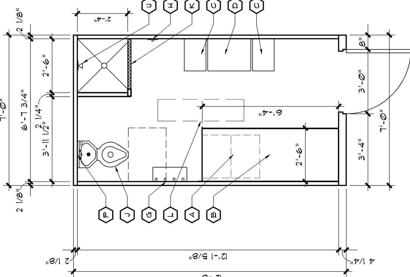
Indirect Supervision Standard Cell
