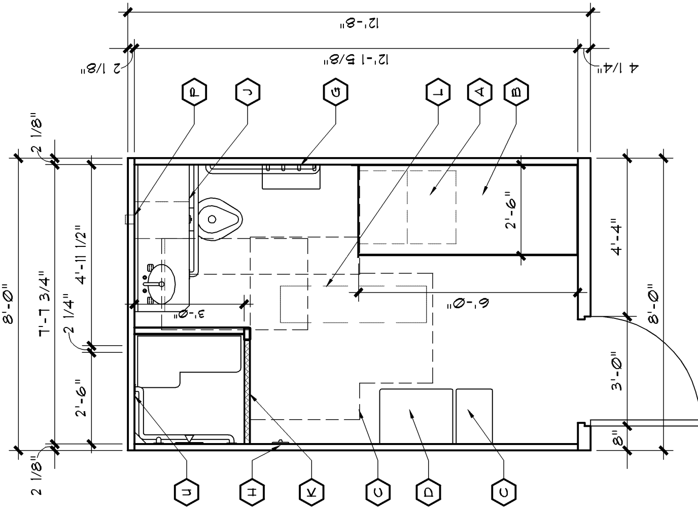
Indirect Supervision Standard Cell
