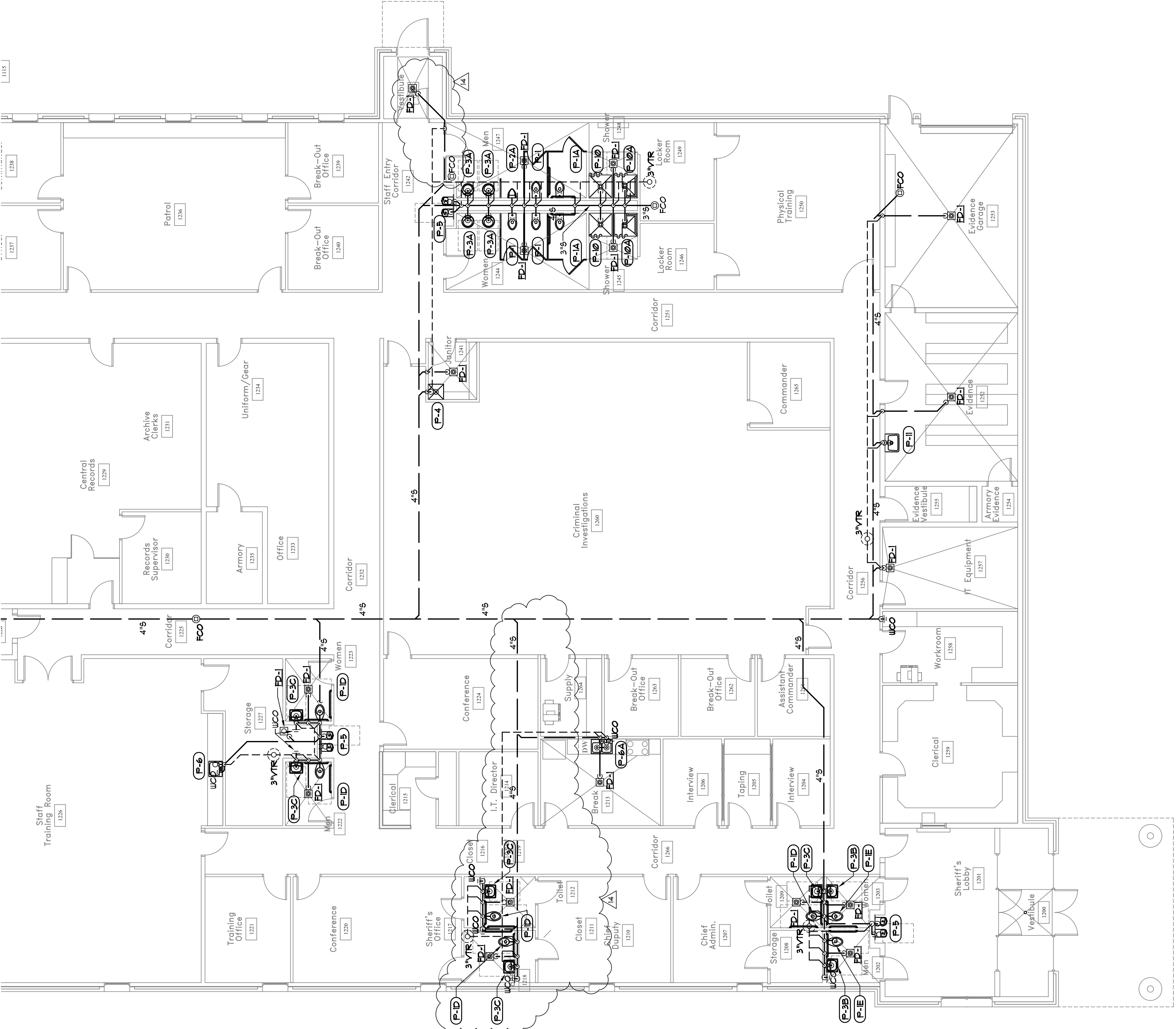
1 PLUMBING PLAN DWV - Area 'A' SCALE 1/8" = 1'-0"
