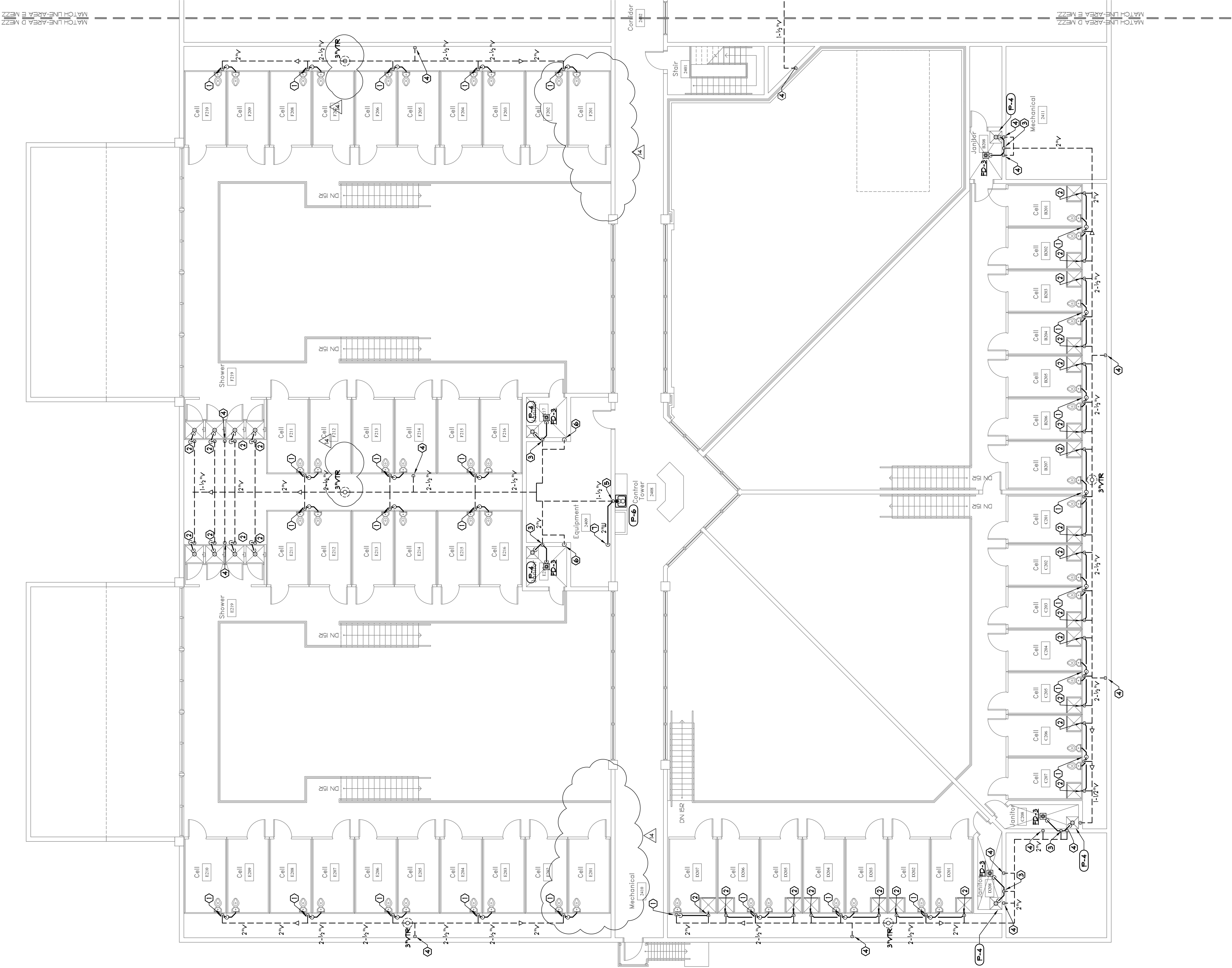
1 PLUMBING PLAN - Area 'D' - Mezzanine P-15 SCALE 1/8\"/>
