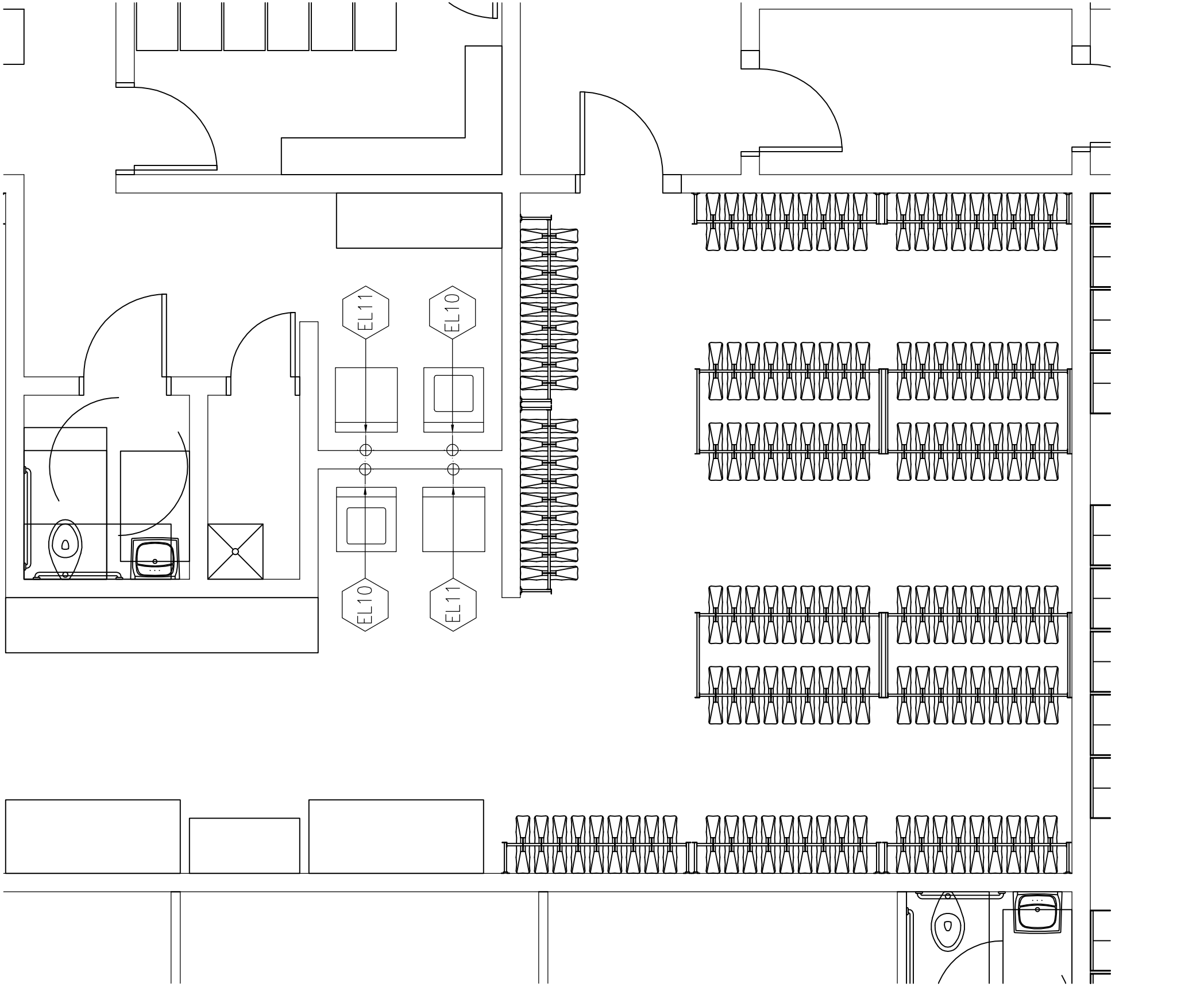
2 MEDICAL/INMATE PROPERTY LAUNDRY EQUIPMENT ELECTRICAL PLAN L3.1 SCALE: 1/4" = 1'-0"
