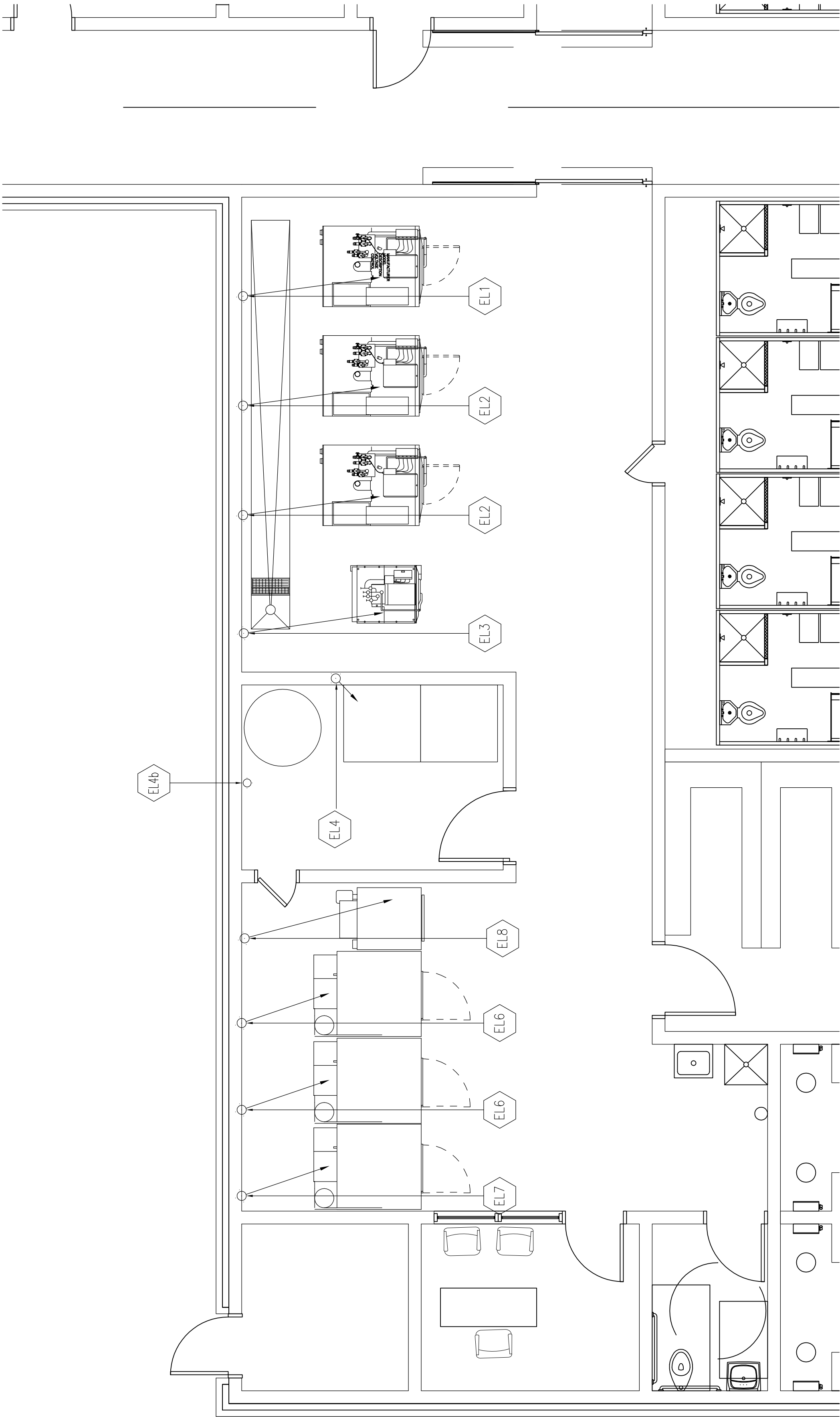
1 LAUNDRY EQUIPMENT ELECTRICAL PLAN L3.1 SCALE: 1/4" = 1'-0"
