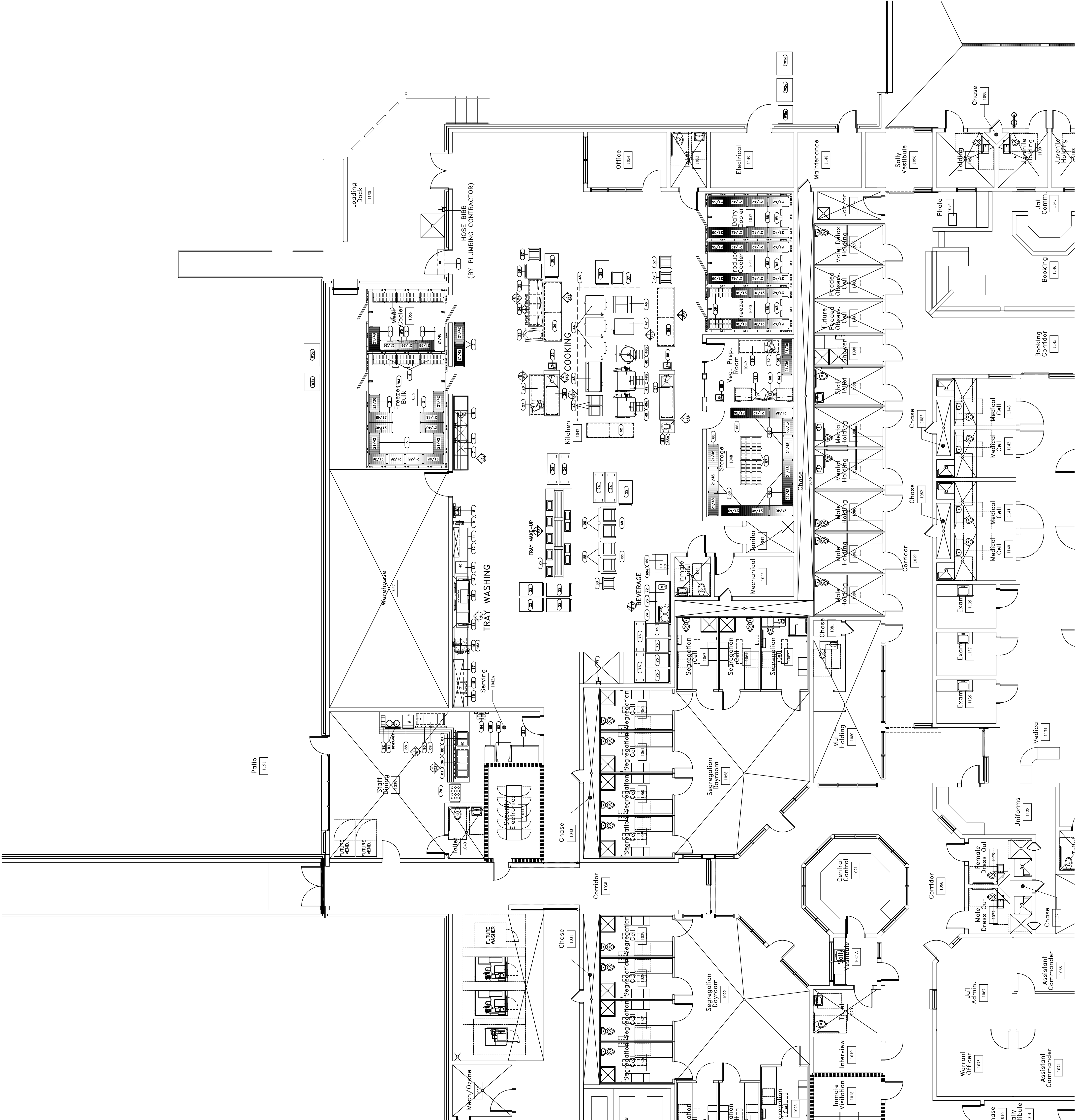
1 KITCHEN EQUIPMENT FLOOR PLAN K1.1 SCALE: 1/8" = 1'-0"
