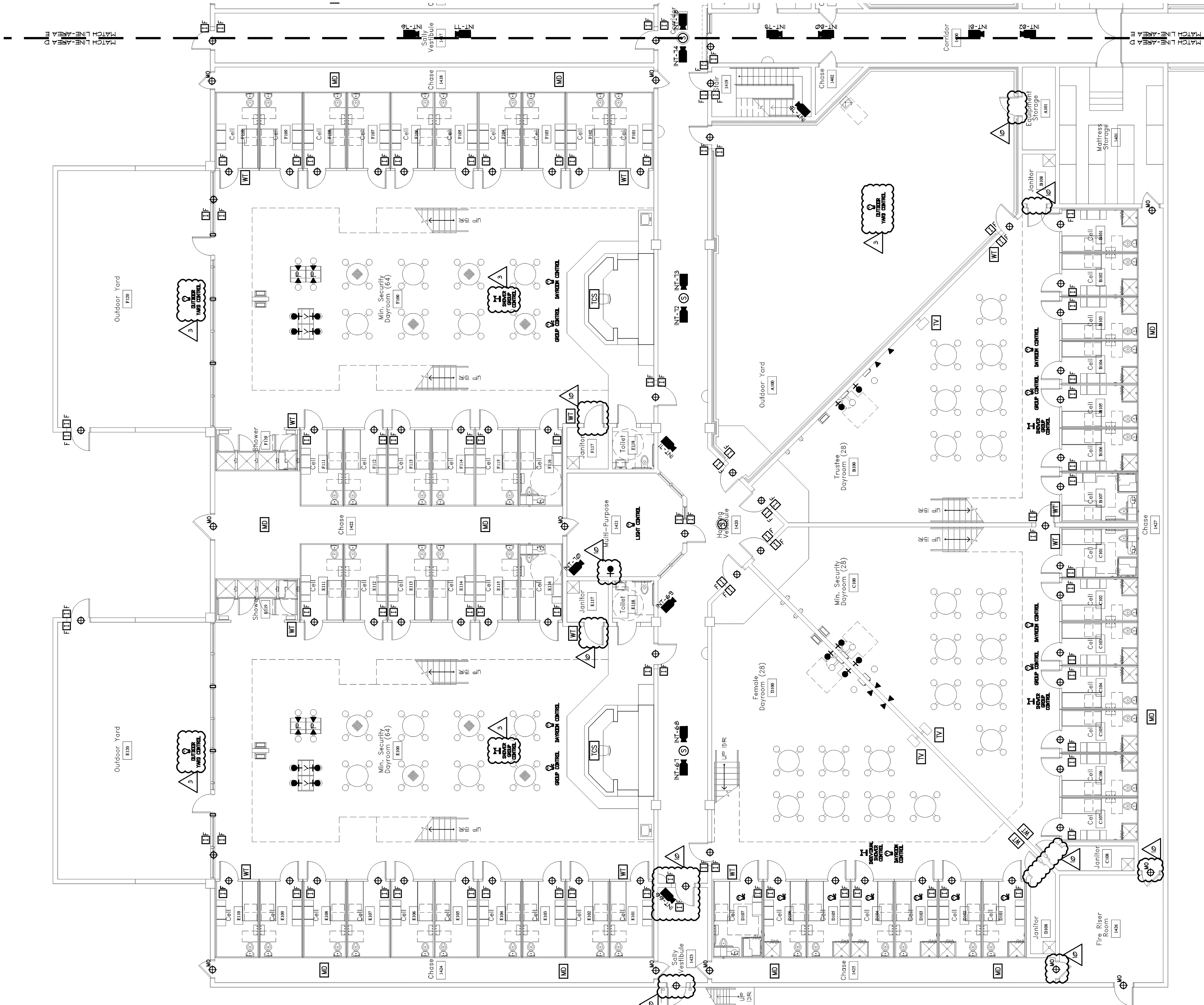
Security Electronics Plan - Area "D"
