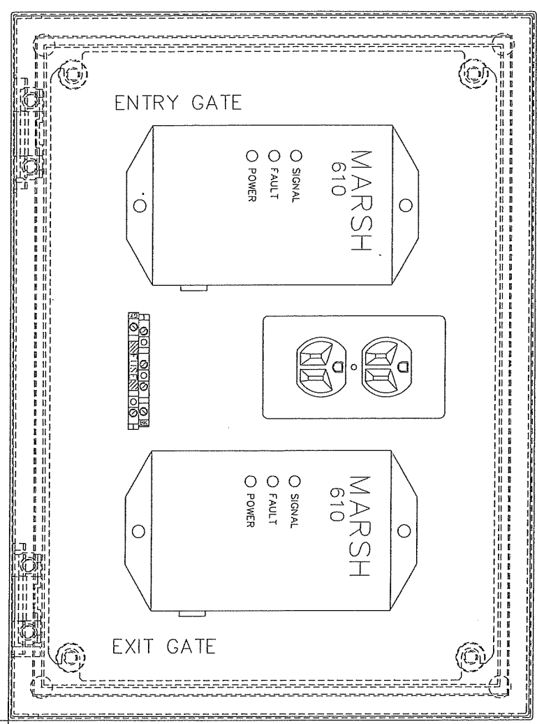
TYPICAL GATE (x2)
