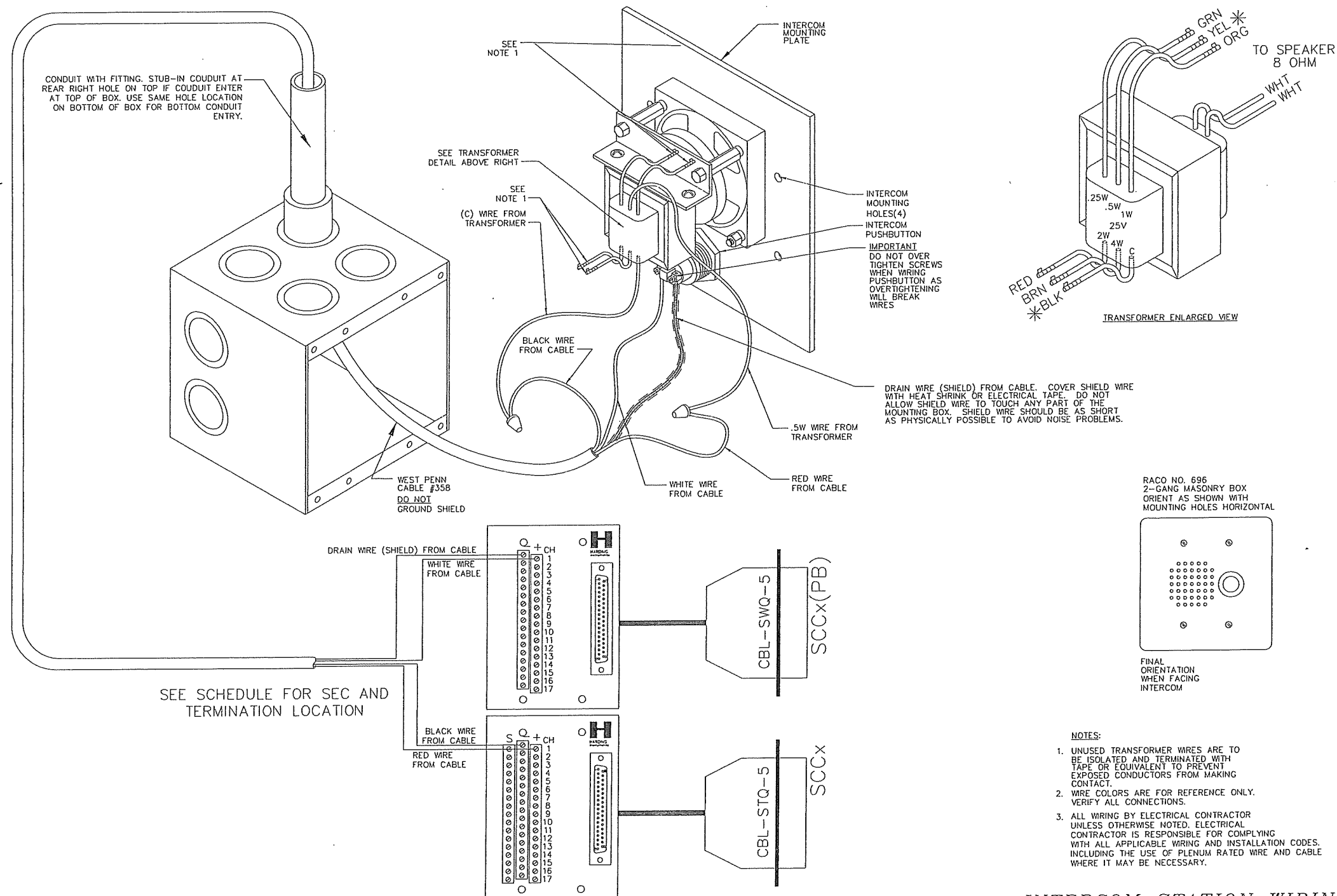
INTERCOM STATION WIRING DIAGRAM
