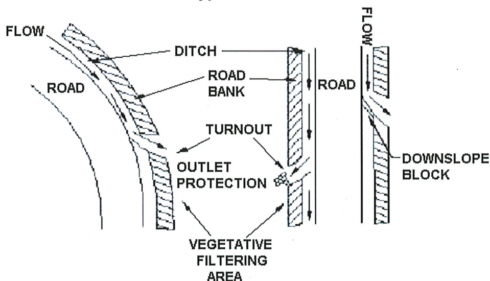
FIGURE 3.3 Typical Turnout
