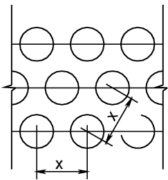
SHRUB BED PLANTING DETAIL
