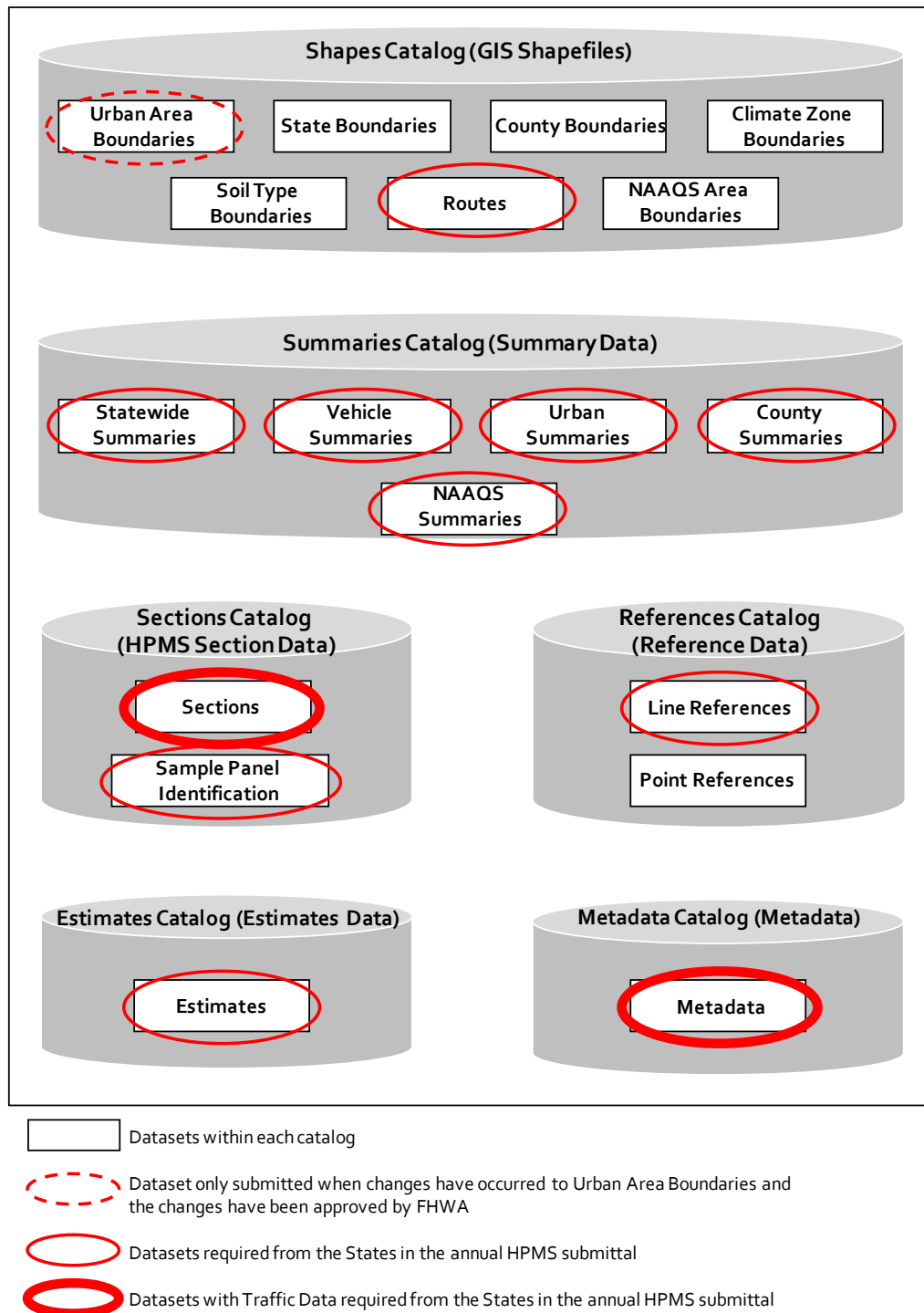
FIGURE 6-2 HPMS DATA MODEL STRUCTURE
