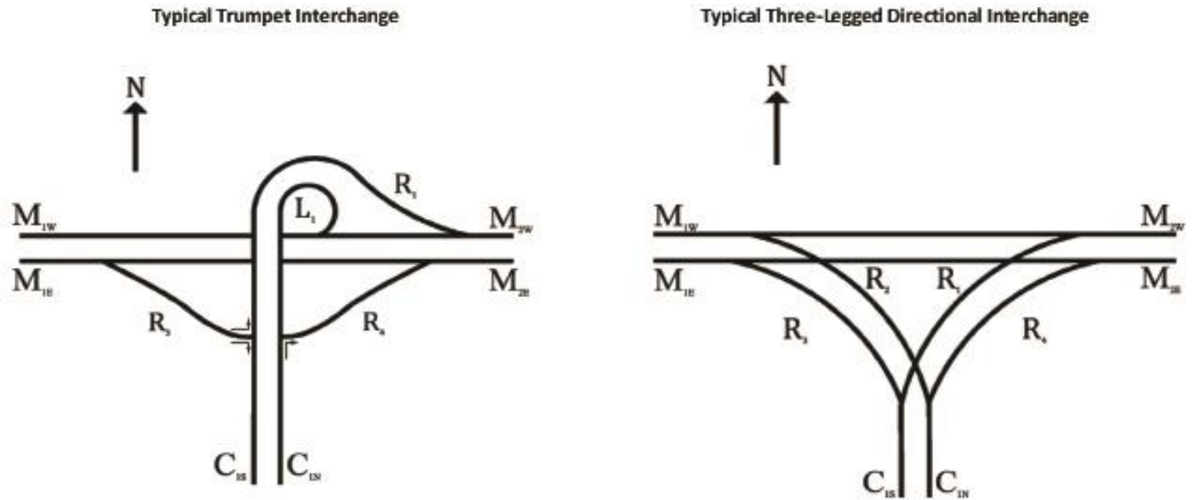
FIGURE 6-5 TYPICAL TRUMPET AND THREE-LEGGED DIRECTIONAL INTERCHANGES
