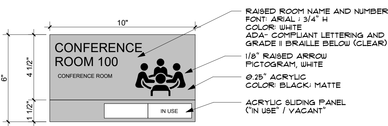
E SIGN TYPE E- SLIDER 3" = 1'-0"
