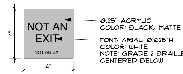
L SIGN TYPE L - NOT AN EXIT 3" = 1'-0"
