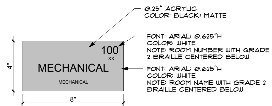
C SIGN TYPE C - GENERAL (SMALL) 3" = 1'-0"
