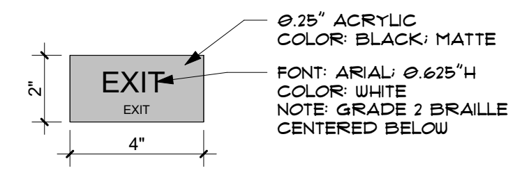
J SIGN TYPE J - EXIT 3" = 1'-0"
