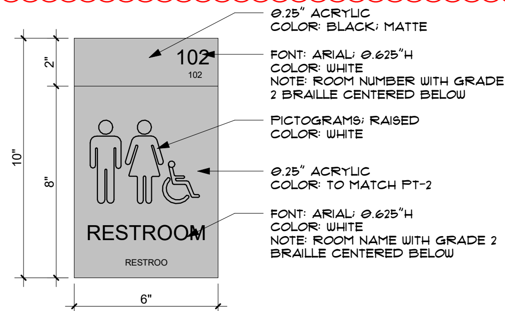
H SIGN TYPE H - EXTERIOR SEAL 3" = 1'-0"
