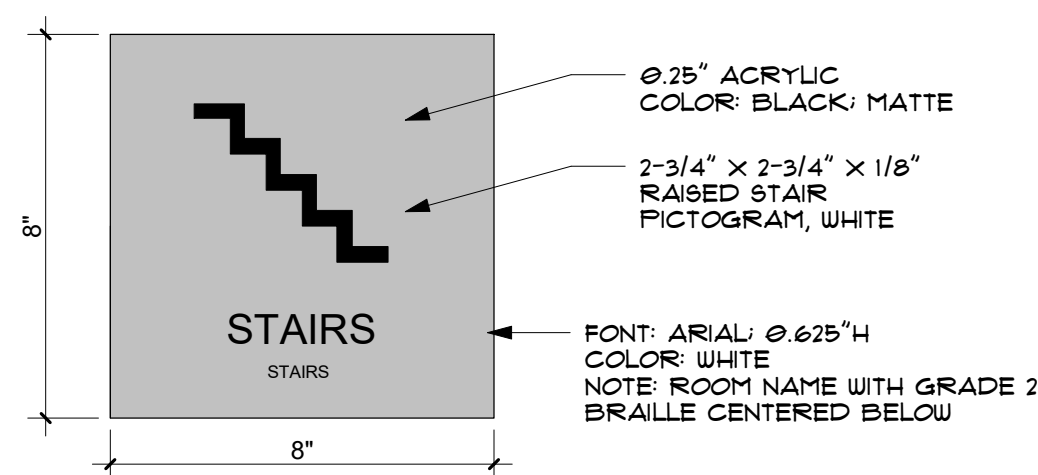
F SIGN TYPE F - STAIR 3" = 1'-0"
