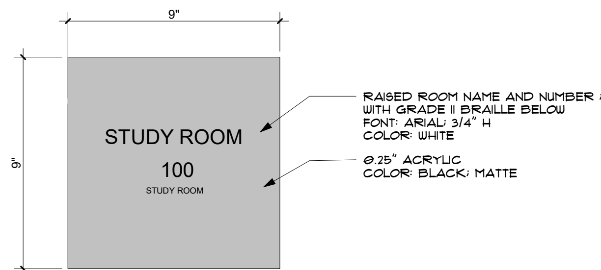
A SIGN TYPE A - GENRAL 3" = 1'-0"
