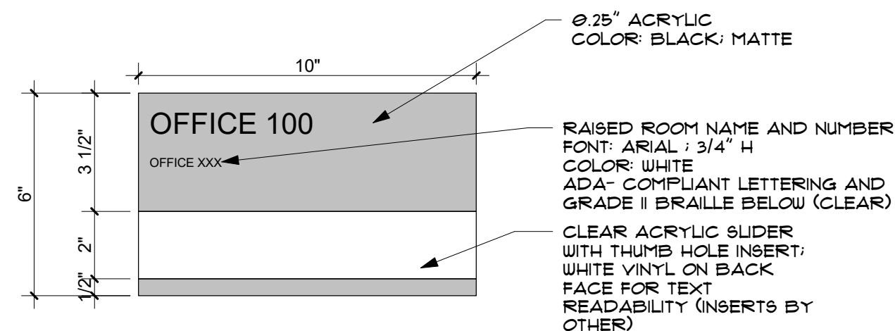
B SIGN TYPE B - OFFICE 3" = 1'-0"
