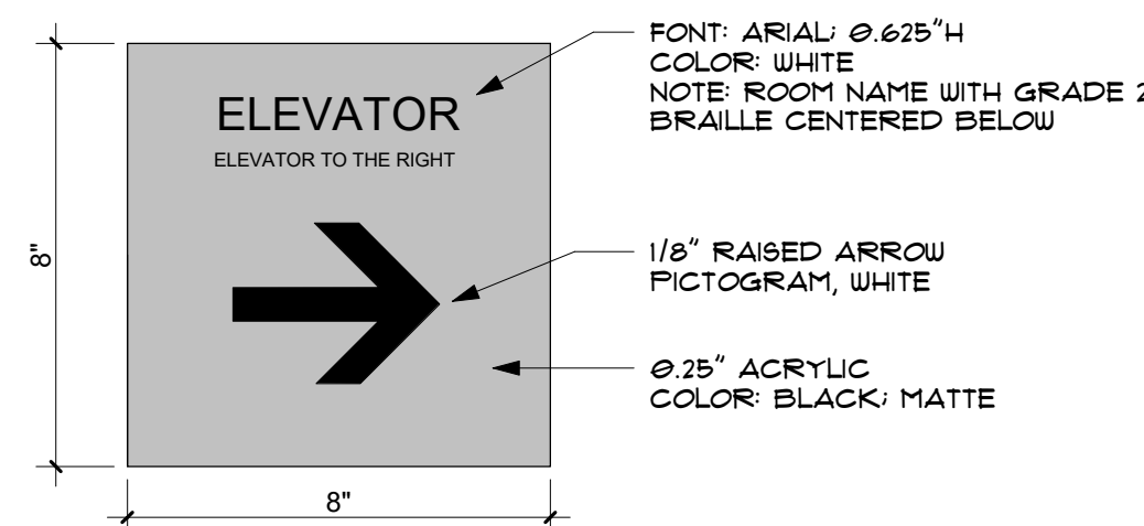
G SIGN TYPE G - ELEVATOR 3" = 1'-0"
