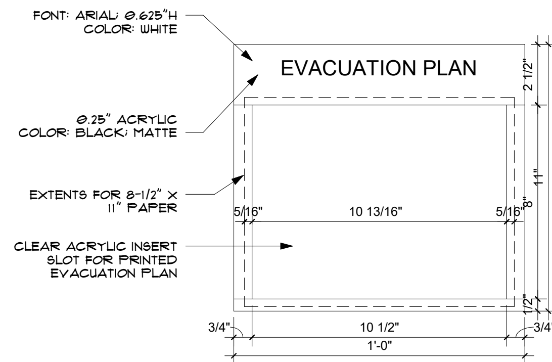
M SIGN TYPE M - EVACUATION PLANS 3" = 1'-0"
