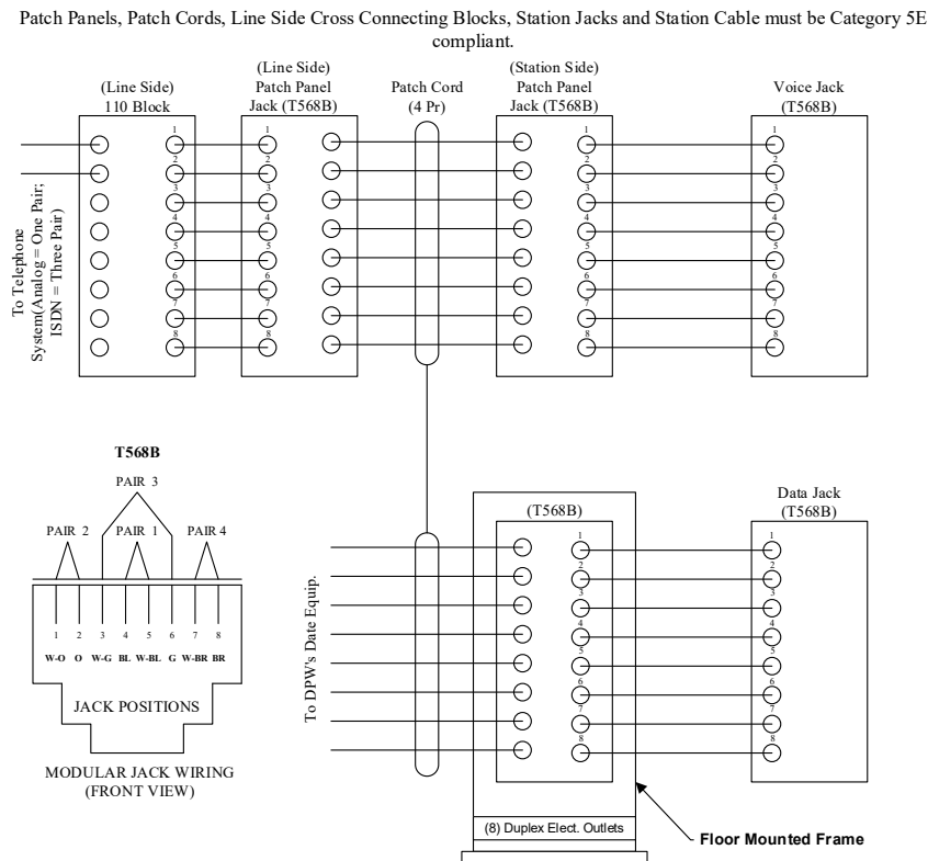
Wiring Diagram
